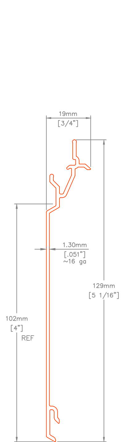
P44V V-NOTCH 4" PLANK
