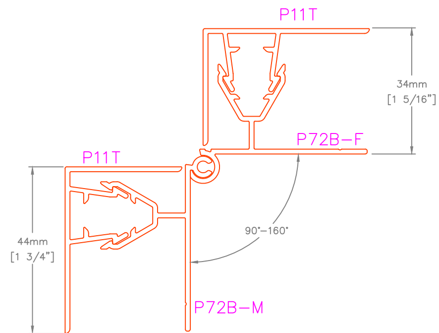
P72 ADJUSTABLE OUTSIDE CORNER
