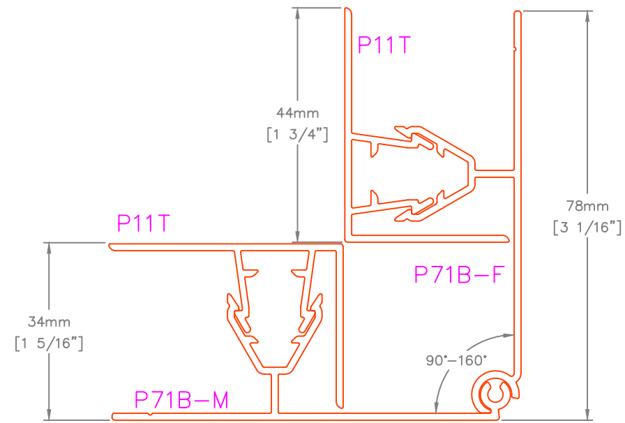
P71 ADJUSTABLE INSIDE CORNER
