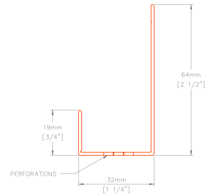
P41 PERFORATED STARTER J
