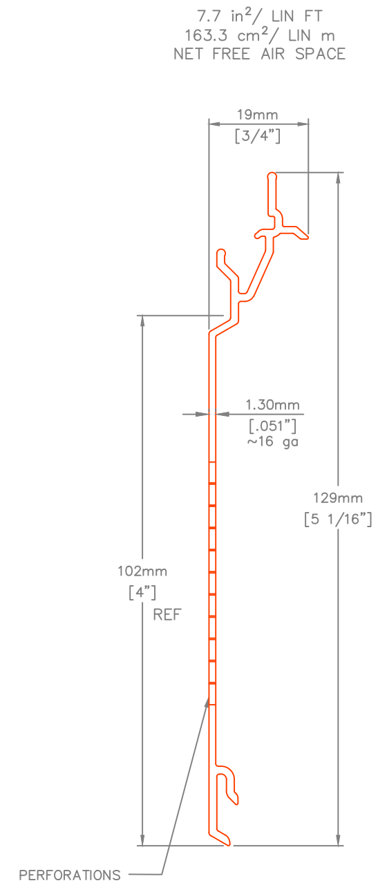
P47V V-NOTCH SOFFIT PLANK
