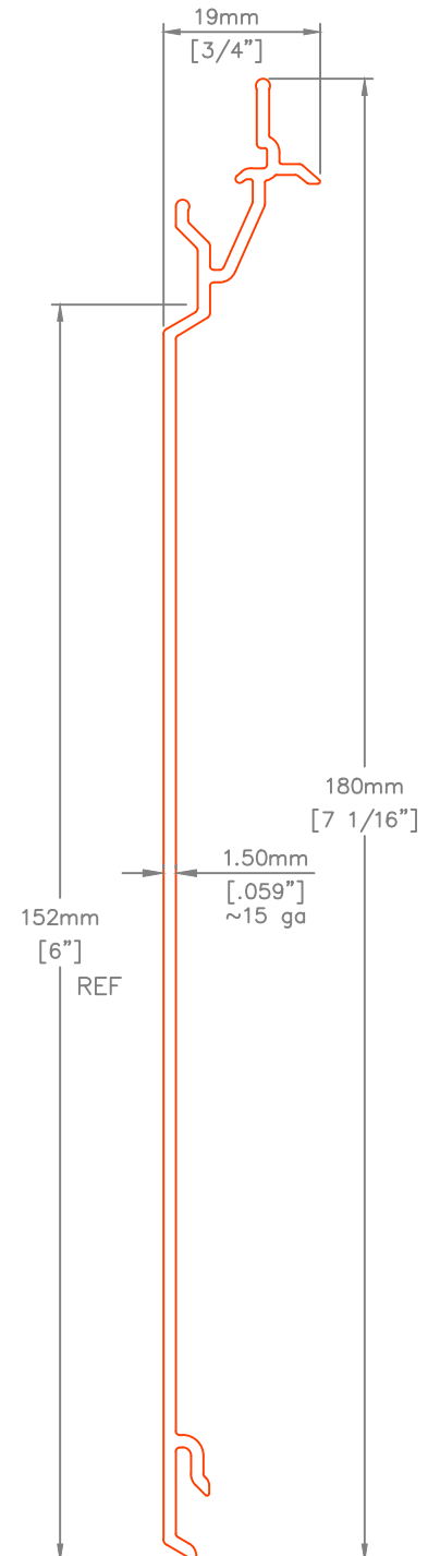
P46V V-NOTCH 6" PLANK
