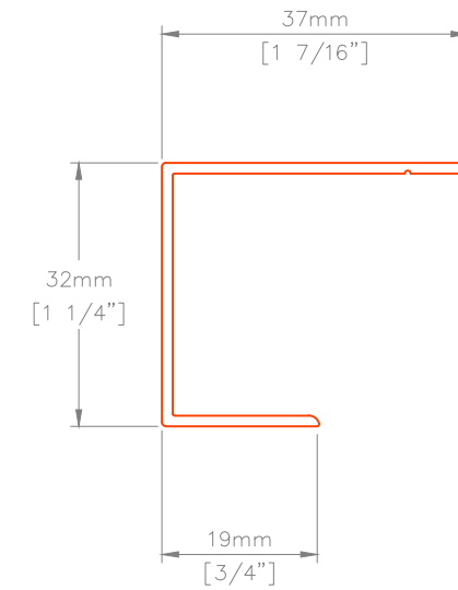
P13 GENERAL J
