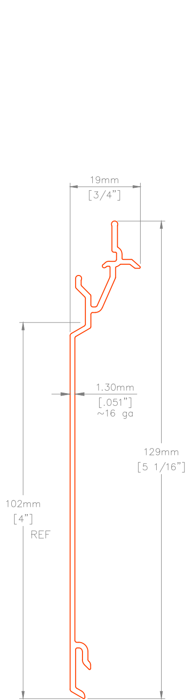
V 4.1.4" V-NOTCH 4" PLANK
