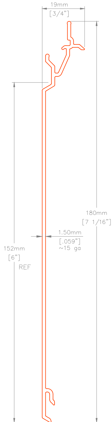
V 4.1.6" V-NOTCH 6" PLANK
