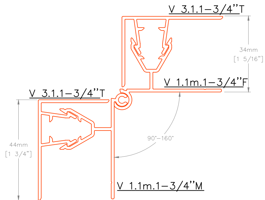
V 1.1m.1-3/4\" MULTI-ANGLE OUTSIDE CORNER
