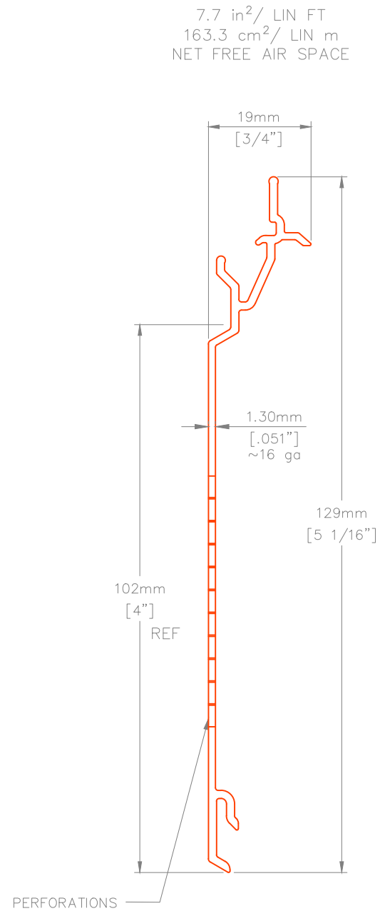
V 4.0ps.4" 4" PERFORATED SOFFIT PLANK
