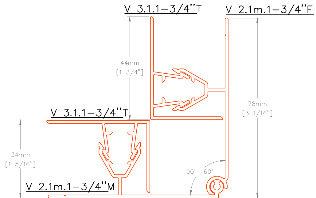
V 2.1m.1-3/4\" MULTI-ANGLE INSIDE CORNER
