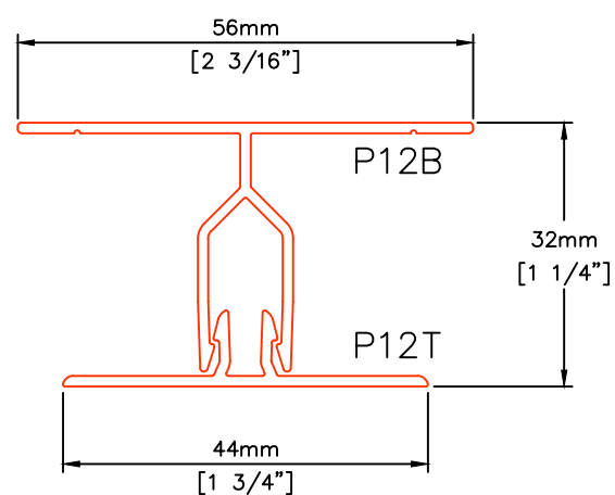
P12 2-PIECE VERTICAL
