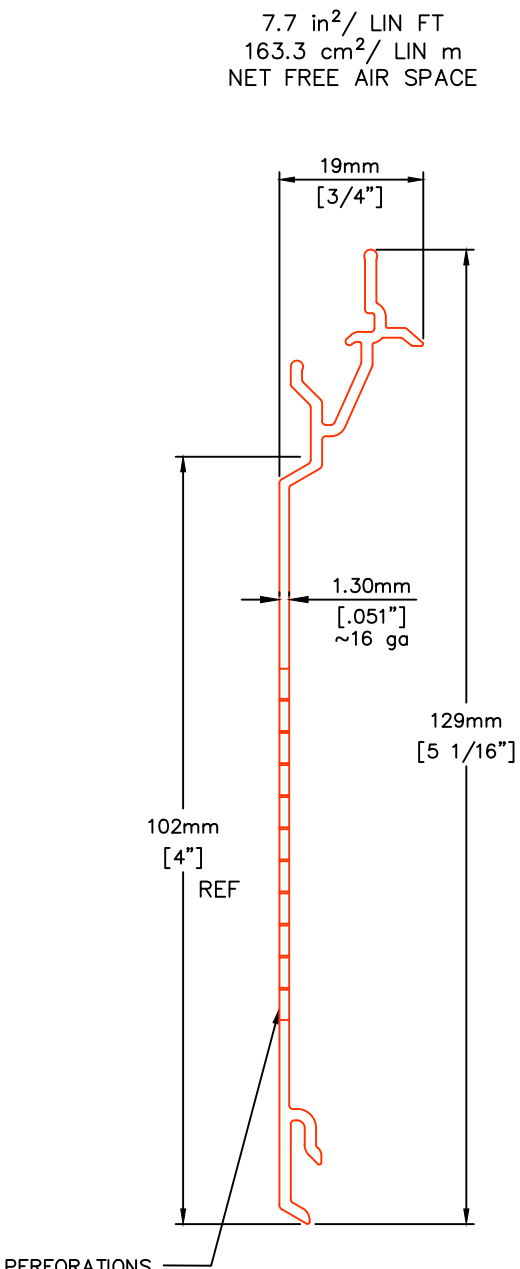
P47V V-NOTCH SOFFIT PLANK
