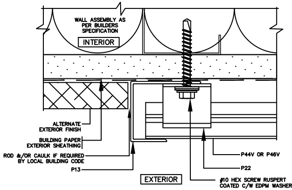
C 5 — GENERAL J VERTICAL TERMINATION NOT-TO-SCALE | PLAN
