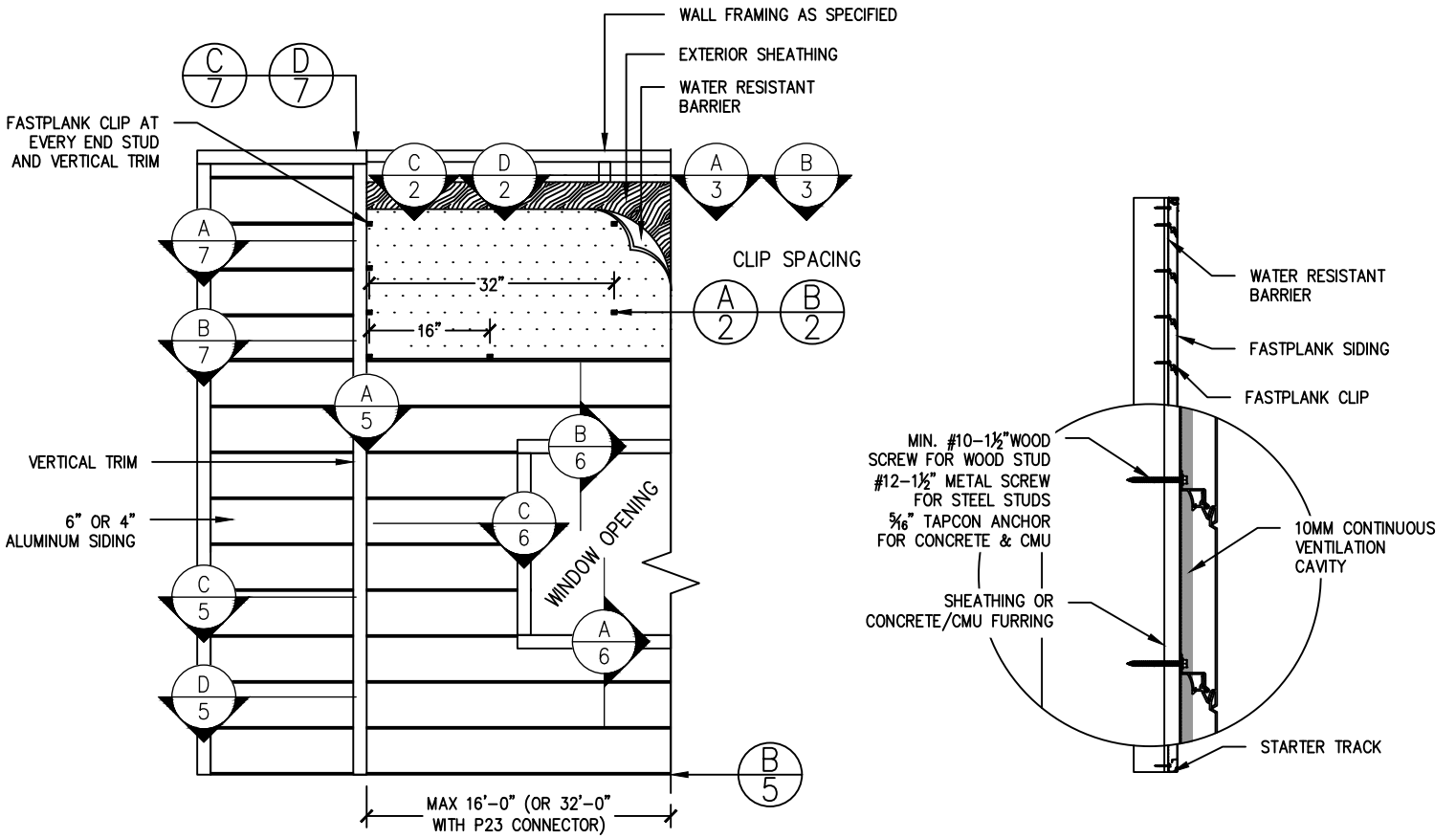
A 1 FASTPLANK WALL ELEVATION NOT-TO-SCALE | ELEVATION
