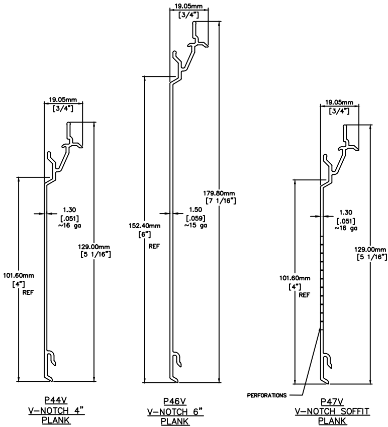
A 4 FASTPLANK V-NOTCH SIDING PLANKS NOT-TO-SCALE
