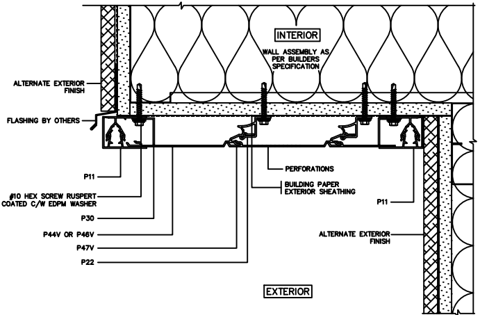
D 8 SOFFIT W/ 2-PIECE J TRIM DETAIL II NOT-TO-SCALE | ELEVATION
