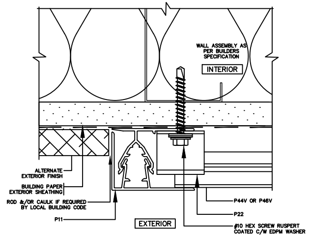
D 5 — 2-PC J VERTICAL TERMINATION NOT-TO-SCALE | PLAN
