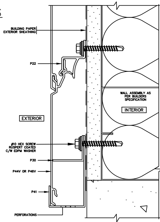
B 5 — PERFORATED STARTER J TRIM NOT-TO-SCALE | ELEVATION
