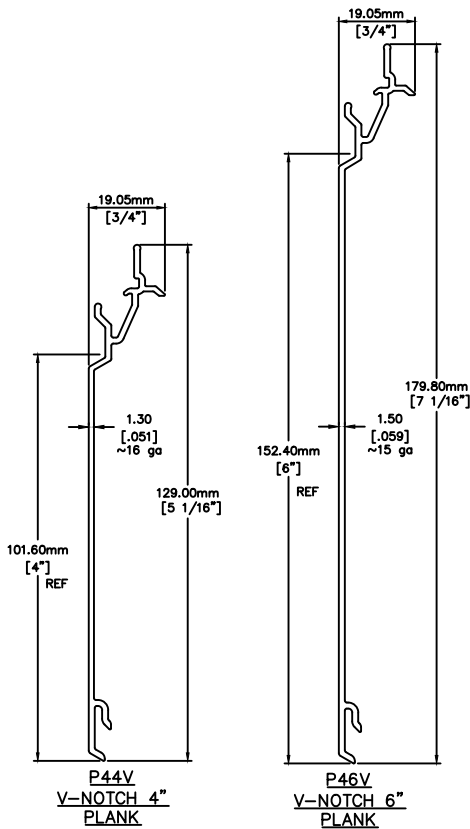
A 3 FASTPLANK V-NOTCH SIDING PLANKS NOT-TO-SCALE
