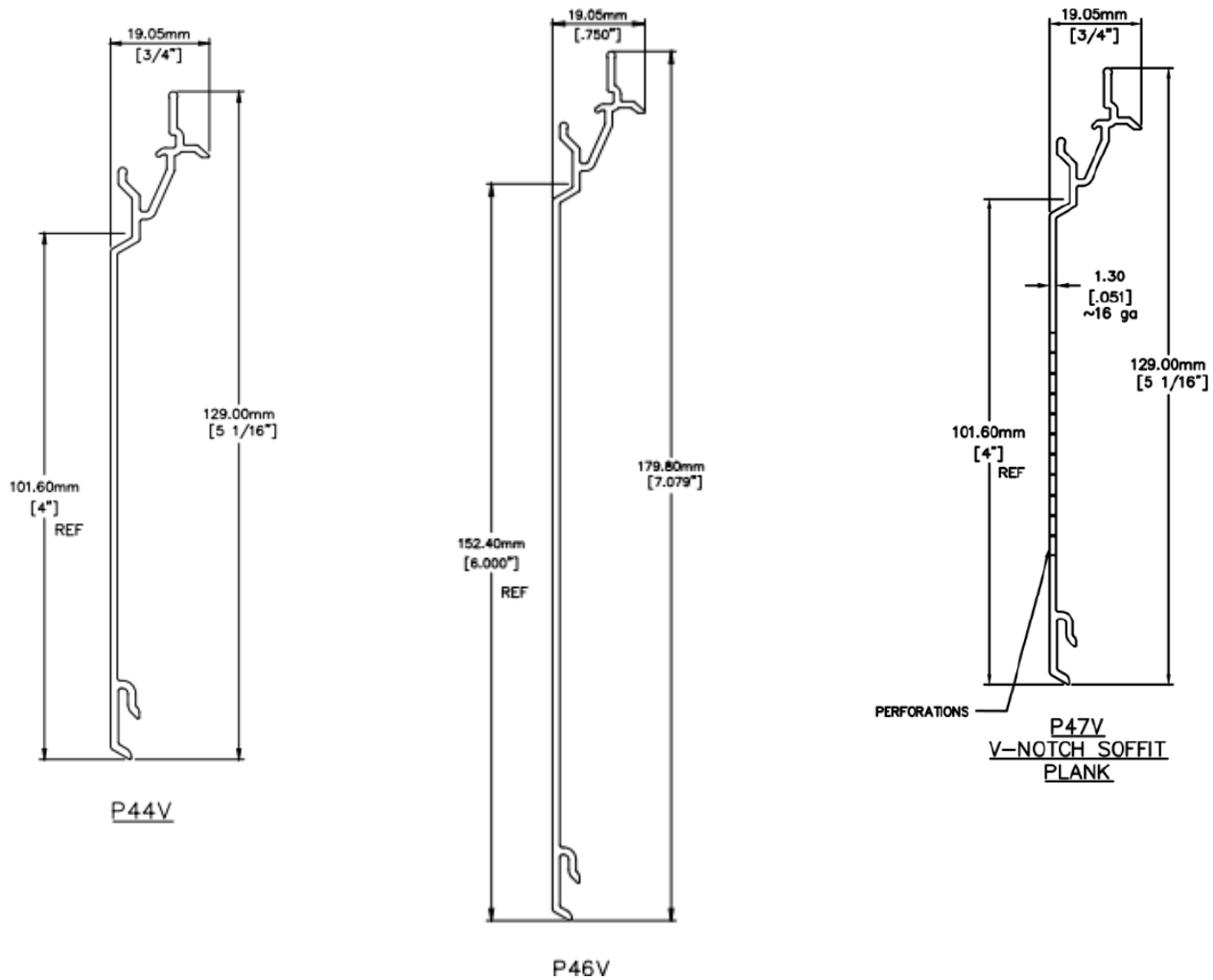
FIGURE 1 – PLANK DIMENSIONS
