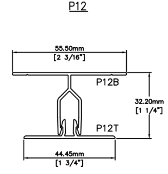
H VERTICAL TRIM 4 NOT-TO-SCALE
