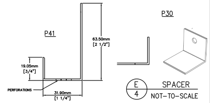
D PERFORATED STARTER TRACK 4 NOT-TO-SCALE E SPACER 4 NOT-TO-SCALE
