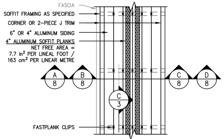
D 1 CLIPS AT 24" O.C STRAIGHT NOT-TO-SCALE | BOTTOM VIEW
