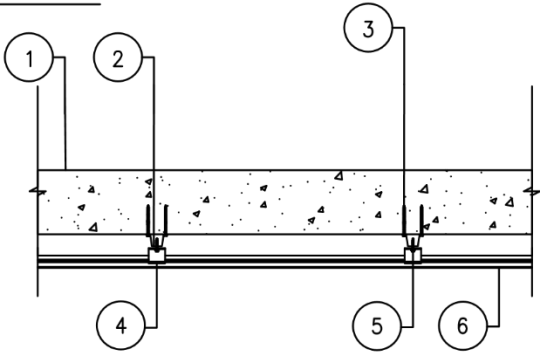
A 3 FASTPLANK OVER CONCRETE WALL NOT-TO-SCALE | PLAN
